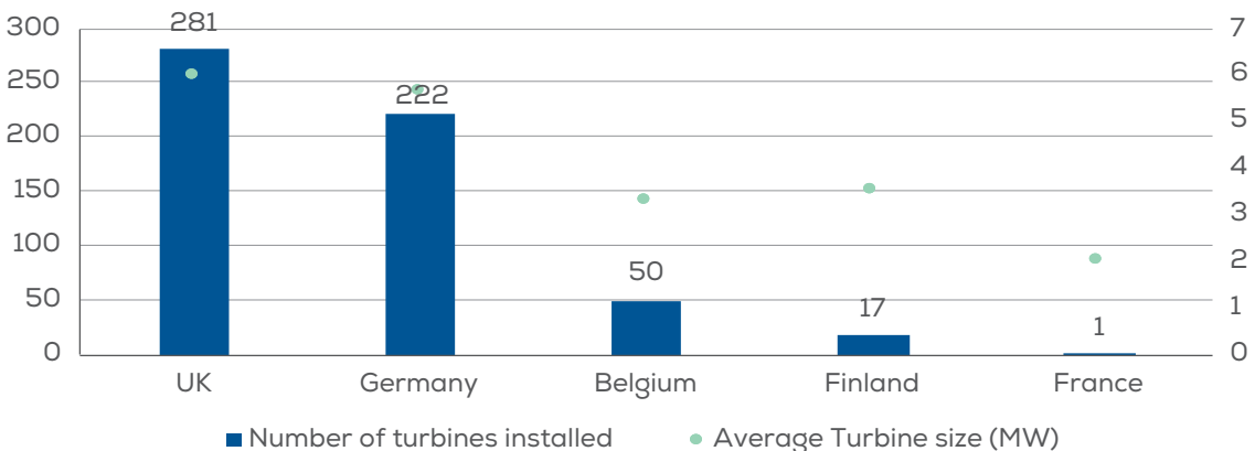
FIGURE 16 Number of turbines installed in 2017 and their average power rating – Offshore
